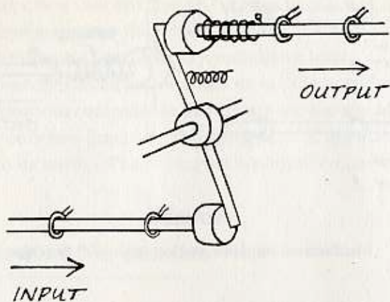
FIGURE 5 Mechanical inverter
